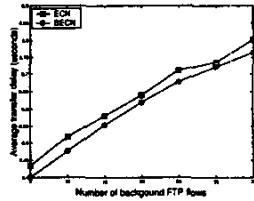
Fig. 9. Average object transfer delay
