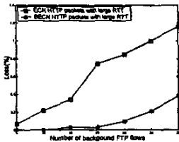
Fig. 18. HTTP data packet loss
