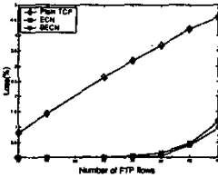
Fig. 5. Loss - Homogeneous flows
