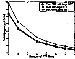
Fig. 11. Goodput - Homogeneous flows
