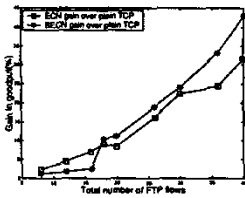
Fig. 2. Goodput gain over TCP
