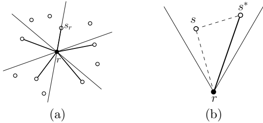
Figure 3: (a) s_r is the nearest neighbor of r which is shared between two cones; bold edges are added to G' . (b) The edge (r, s^*) \in T_{opt} is replaced by two edges (r, s) and (s, s^*) .
