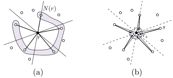
Figure 4: (a) neighbors of a terminal r in G' , (b) group g_r of the copies of a terminal r in G'' .
