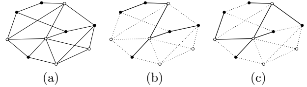
Figure 1: (a) the input graph G ; terminals are black, non-terminals are white, (b) a Steiner tree, and (c) a full Steiner tree of G .
