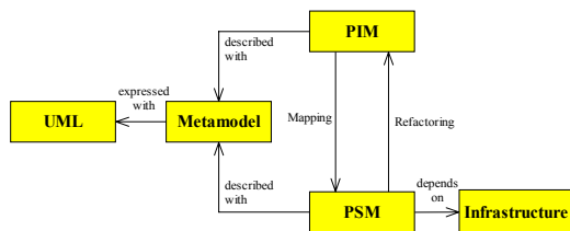
Figure 3. Model driven development.
