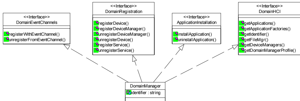
Figure 9. The DomainManager class.
