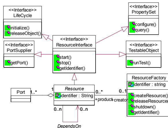
Figure 6. Class diagram of Base Application.
