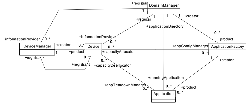
Figure 7. Class diagram for Application and Device.
