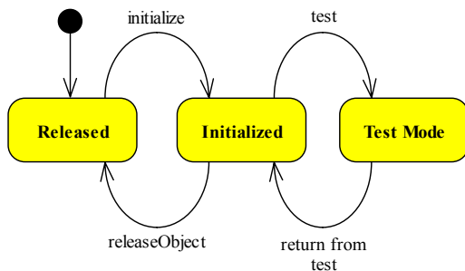
Figure 5. Statechart diagram for Resource instance.
