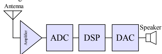
Figure 1. Architecture of a SWR receiver.
