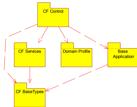
Figure 4. Package view of a SWR.
