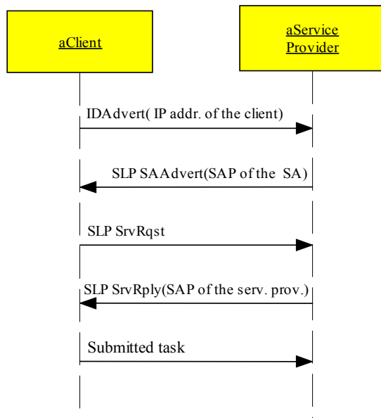
Figure 2. The IDAdvert protocol.
