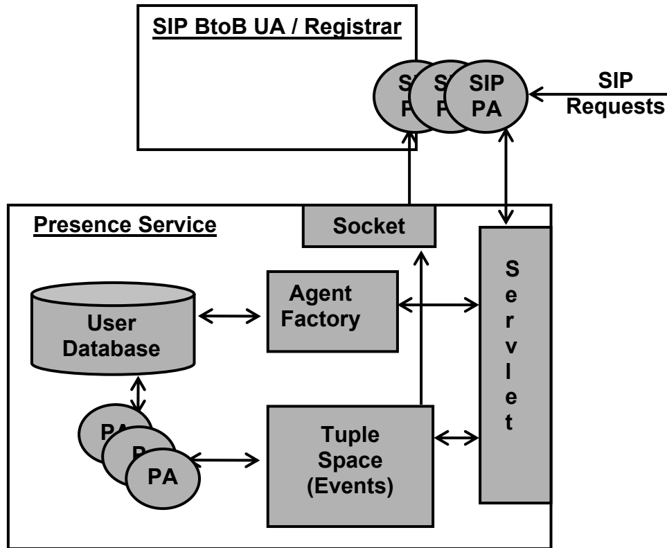
Figure 5. Components of the presence service.
