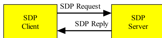
Figure 1. SDP Client-server Interaction.
