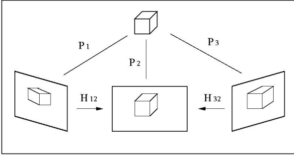
Figure 2. Homographic parameterization
