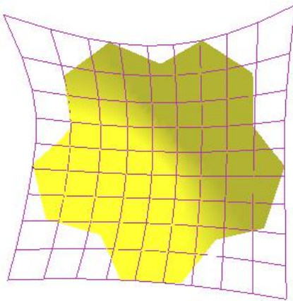
Figure 4. Fitting result of a degree 2 B-spline surface
