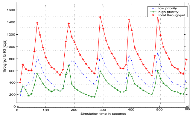
Fig. 4. Throughput for Receiver R3
